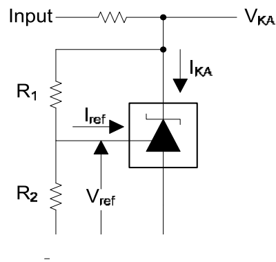
Test Circuit for V_{KA} = V_{ref}(1 + R_1/R_2) + R_1 \cdot I_{ref}
